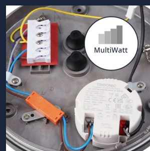
MULTIWATT TRIDONIC Multiwatt driver
