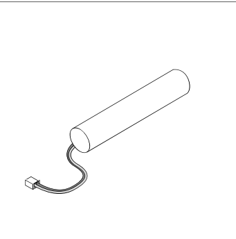
1023298 V: 3,2 mAh: 1500 Afmeting: 65.15x18.5mm Cells: IFR18650-1500 Connector: HX25002-3Y 60mm
